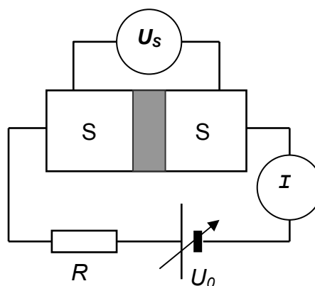
Fig. 5: Josephson junction
