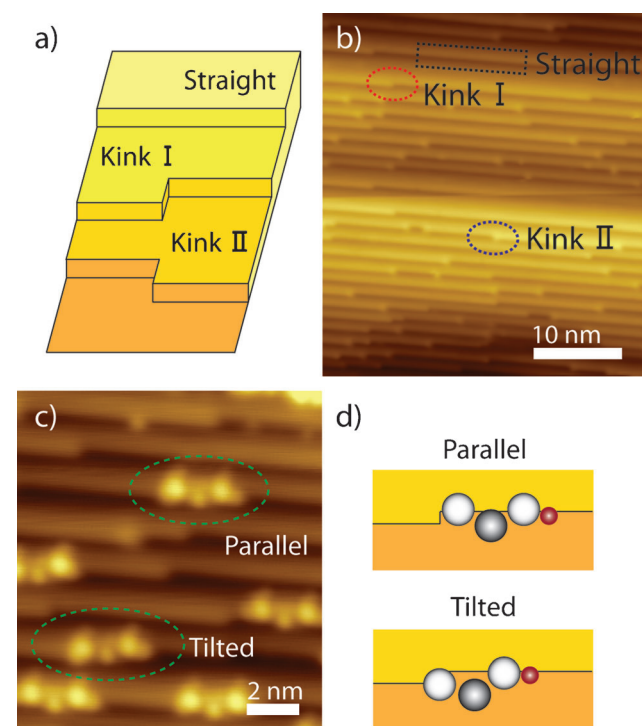
Figure 3. a) Scheme showing the two types of step-edge kinks present on the surface and a straight region of the step edge. b) STM image showing examples of the kink I and kink II step-edge defects ( V_{\text{tip-bias}} = +200 mV, I_{\text{tunnel}} = 1.00 nA). c) STM image showing several DBTF molecules adsorbed at kink I sites ( V_{\text{tip-bias}} = -600 mV, I_{\text{tunnel}} = 0.55 nA), highlighted molecules adsorbed at kink I sites have had their 'left' Br atom dissociated. d) Scheme showing molecules in parallel and tilted orientations at a kink I step-edge defect.
