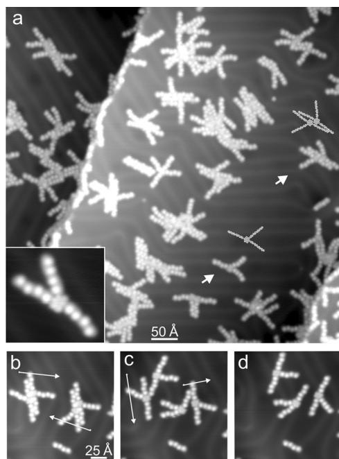
Figure 3. Three-terminal molecular nodes. a) Constant-current STM image ( 686 \times 686 \text{ \AA}^2 , 1 V, 50 pA) taken after dehalogenating the species on the surface. Individual molecular nodes and node clusters were also identified (see arrows and the chemical structures). Inset: STM image (1 V, 50 pA) of an individual three-terminal molecular node. b–d) Untangling of molecular-node clusters by STM-based lateral manipulation. Sequence of constant-current STM images ( 192 \times 189 \text{ \AA}^2 , 1 V, 50 pA) showing molecular nodes untied by constant-current lateral manipulation (set point: 25 mV, 20 nA). The arrows represent the direction along which the manipulation took place. The molecular node manipulated in (c; left) is missing in (d), probably because it was picked up by the STM tip.
