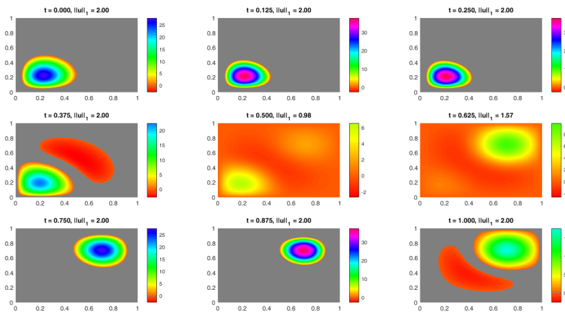
FIG. 2. 2D problem. Piecewise constant approximation of the optimal control. In grey, the level sets \bar{u}_\sigma(\cdot, t_j) = 0 .
