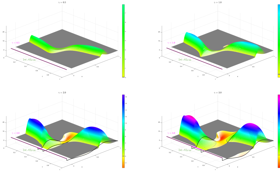
FIG. 1. 1D problem. Continuous piecewise linear approximation in space, piecewise constant approximation in time, of the optimal control for different values of \gamma . The norm in L^1(\Omega) at every instant of time is also shown with a dark green line located on the plane x = -0.1 together with the magenta line z = \gamma . In grey, the zero-level set of \bar{u}_\sigma .
