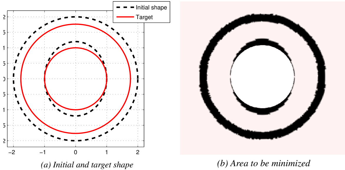
Figure 3: Initial shape \Omega^{(0)} and target shape E
