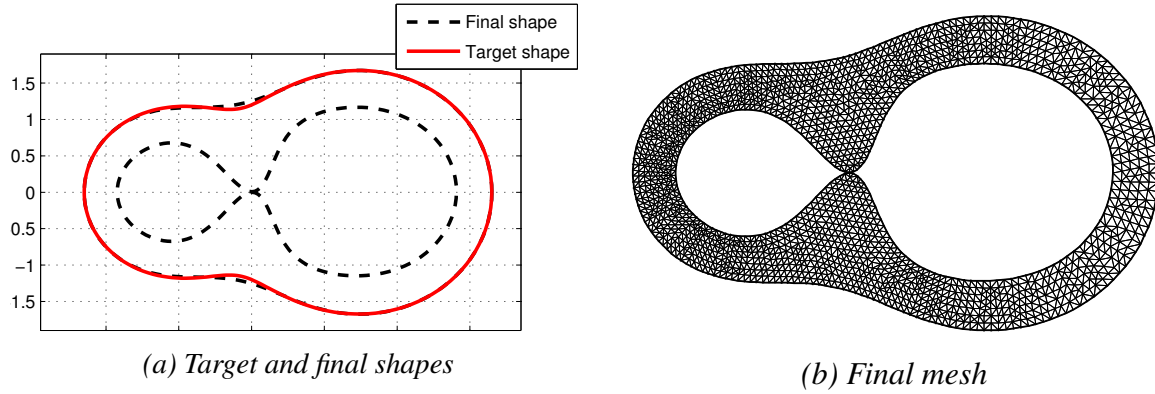
Figure 8: Target shape E and final shapes \omega^{(final)}, \Omega^*(\omega^{(final)}) using K_2 with \mu = -1.8
