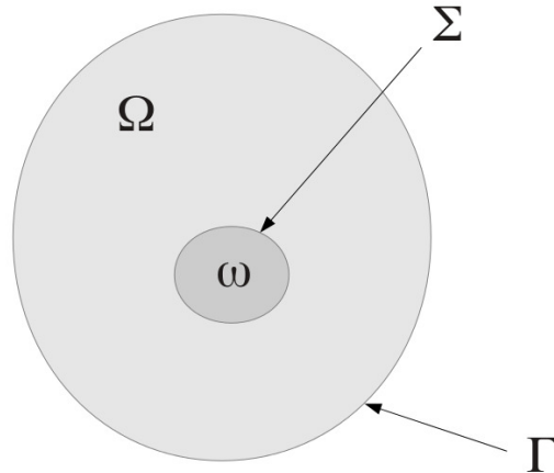
Figure 1: The exterior Bernoulli problem
