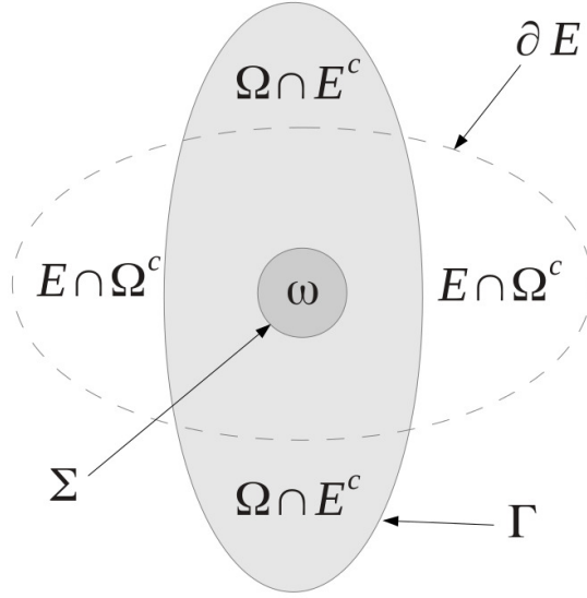
Figure 2: “Free” set \Omega and target E
