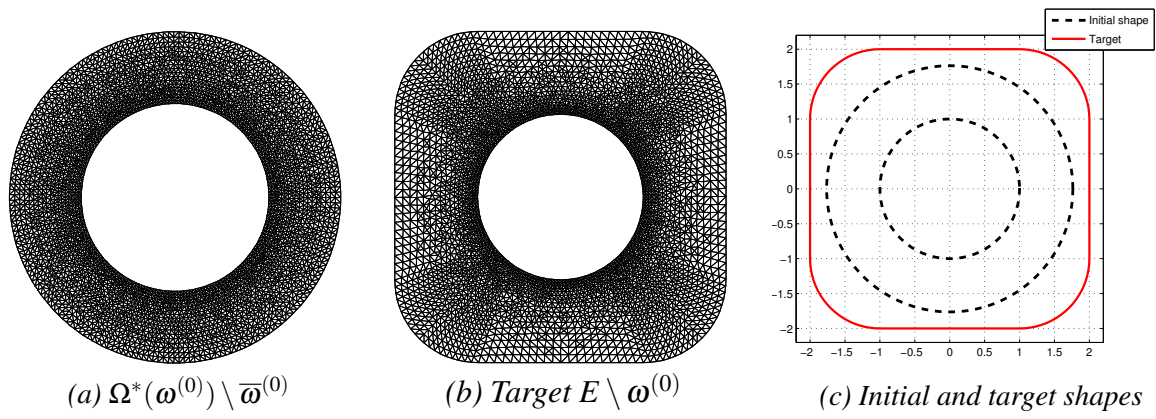
Figure 9: Initial domains and target E
