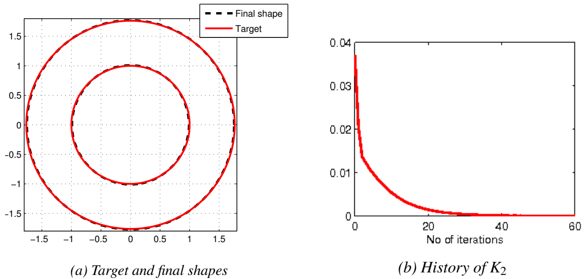
Figure 6: Final shape of the free boundary using K_2 and target shape.
