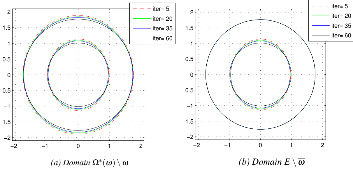
Figure 5: Variations of domains \Omega \setminus \bar{\omega} and E \setminus \bar{\omega}
