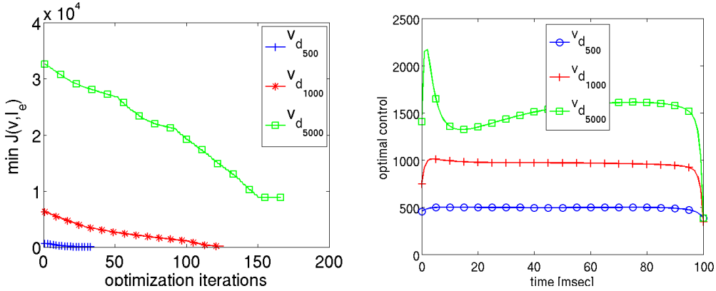
Figure 13: The minimum value of the cost functional and the optimal control values are shown on the left and right respectively for different desired state solutions.
