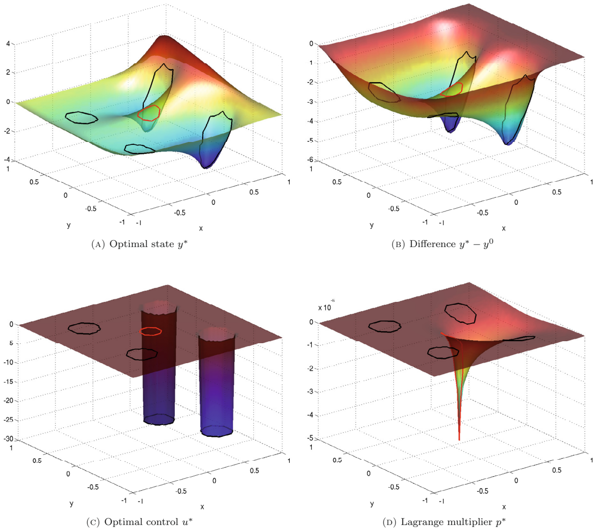
FIGURE 2. Results for unilateral constraint ( y|_{\omega_0} \leq c ).
