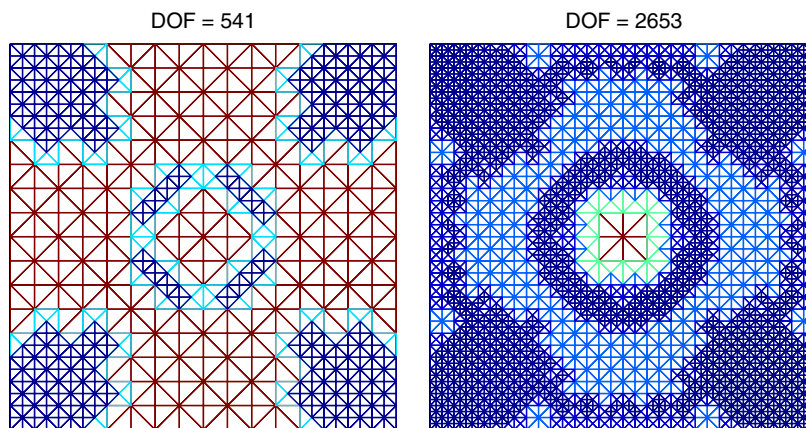
FIG. 4. Adaptive meshes.
