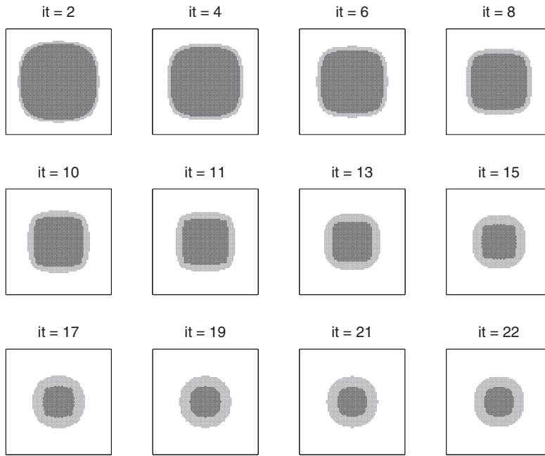
FIG. 3. History of active set iterates.
