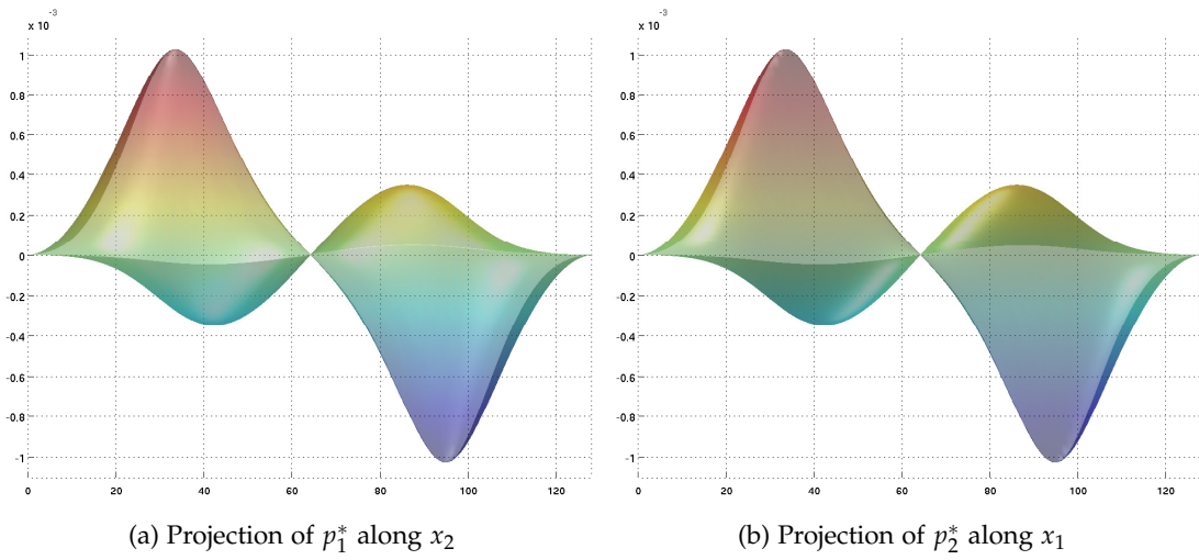
Figure 8: Solution p_b^* = (p_1^*, p_2^*) \in \mathbb{H}_{\text{div}}^2(\Omega) of (\mathcal{P}_{BV,c}^*) with \alpha = 10^{-3} , c = 10^7 .
