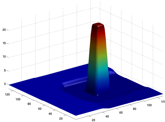
(a) Optimal control u_a^* \in BV(\Omega)
