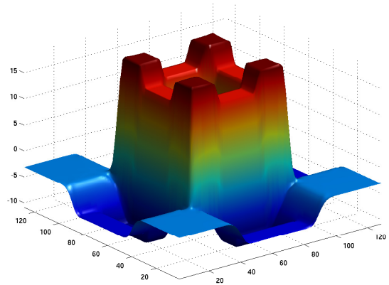
(b) Optimal control u_b^* \in BV(\Omega)
