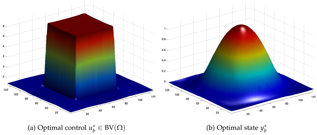
Figure 7: Solution of problem (\mathcal{P}_{BV}) for target z_b with \alpha = 10^{-3} .
