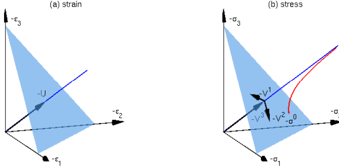
FIG. 3.1. (a) strain space ; (b) stress space
