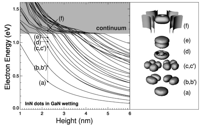
FIG. 1. Electron single-particle energies (left panel) for InN dots GaN [ (x,y)=(1,0) ] as a function of the dot size (60 lowest energy levels); a cylindrical confinement potential is assumed (height/diameter ratio of 1:2.5). The right panel shows the square of the wave functions.
